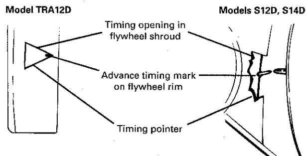
Figure 3 Ignition Timing
