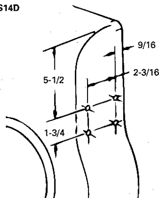
Figure 2 Ignition Module Mounting
