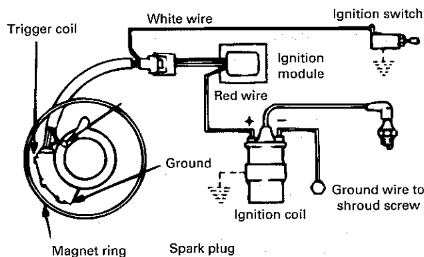
Figure 1 Wiring Diagram
